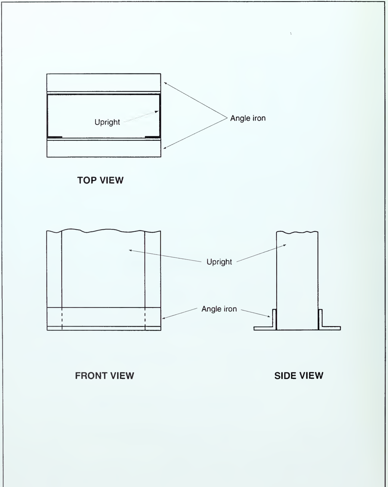
Figure 5. Upright details.
